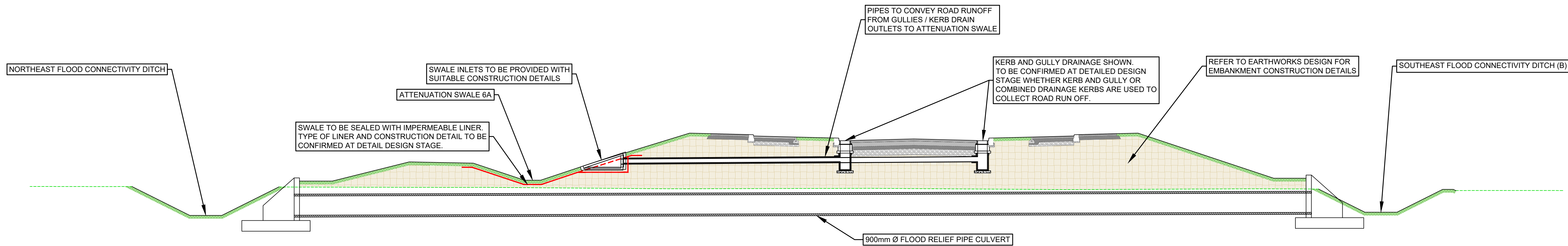
SECTION A - A SCALE 1:100 @A1, SCALE 1:200 @A3
